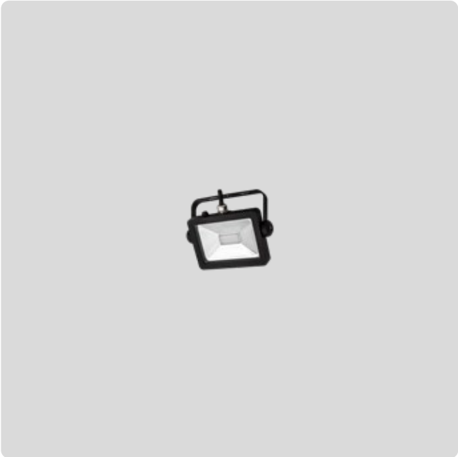
EX300 10W Dimensions L130 x W95 x H21mm Lumens <1020lm Watts 10W Beam 100°
