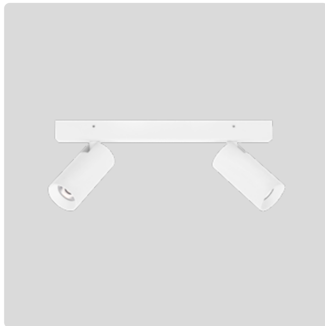
S382 Double Dimensions L350 x W55 x H154mm Spot D55 x L110mm Watts 15W Lumens 2x 650lm Beam 2x 50° Tilt 90° Rotate 350°
