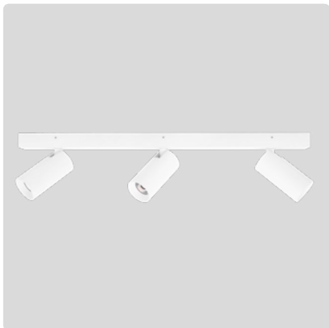
S383 Triple Dimensions L600 x W55 x H154mm Spot D55 x L110mm Watts 20W Lumens 3x 650lm Beam 3x 50° Tilt 90° Rotate 350°
