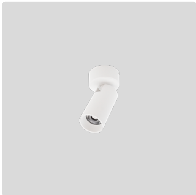
S381 Single Dimensions D75 x L158mm Spot D55 x L110mm Watts 8W Lumens 650lm Beam 50° Tilt 90° Rotate 350°
