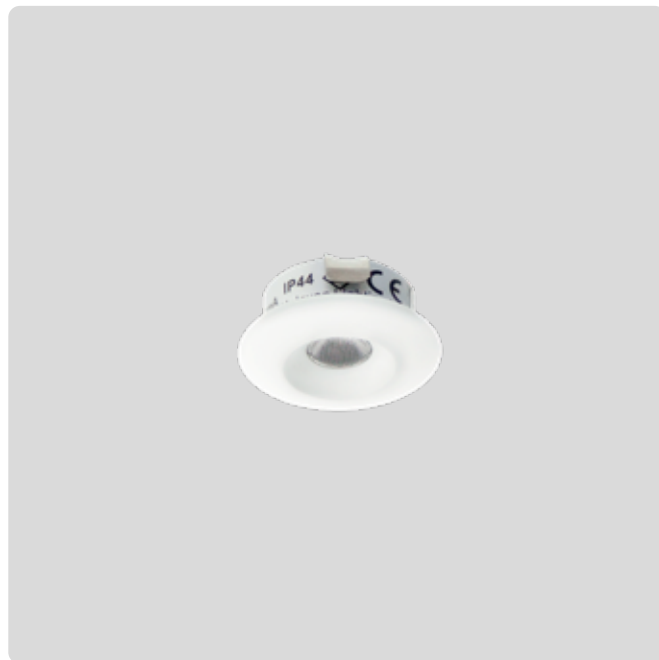
R701 Ultra Shallow Narrow Beam Dimensions D36 x H15mm Cut Out Ø 27mm Watts 1.2W Lumens 95lm Beam 22°
