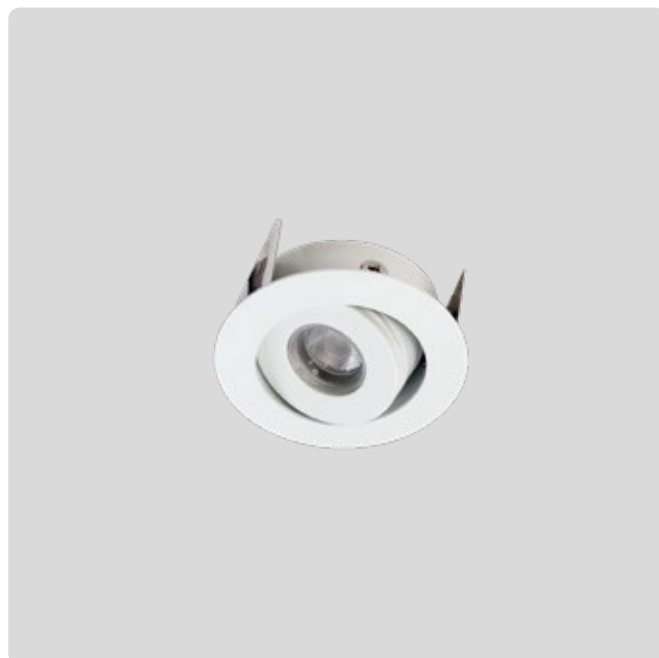
R711 Tilt Wide Beam Dimensions D52 x H22mm Cut Out Ø 46mm Watts 1.2W Lumens 70lm Beam 60° Tilt 30°
