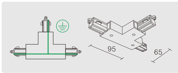
“T” JOIN EARTH RIGHT AC 240V 16A
