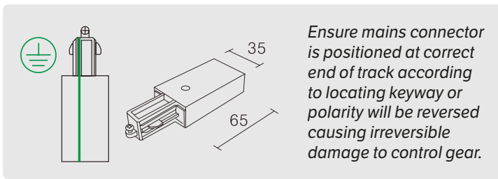
MAINS CONNECTION EARTH LEFT AC 240V 16A
