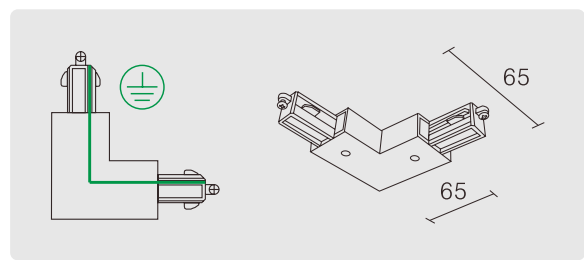
"L" JOIN EARTH INSIDE AC 240V 16A
