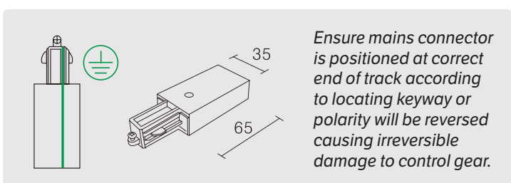
MAINS CONNECTION EARTH RIGHT AC 240V 16A
