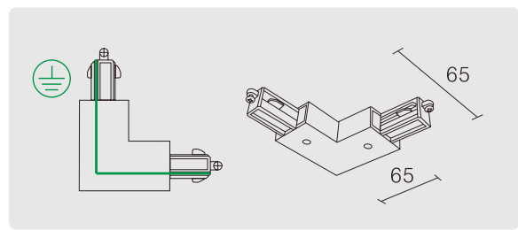
"L" JOIN EARTH OUTSIDE AC 240V 16A
